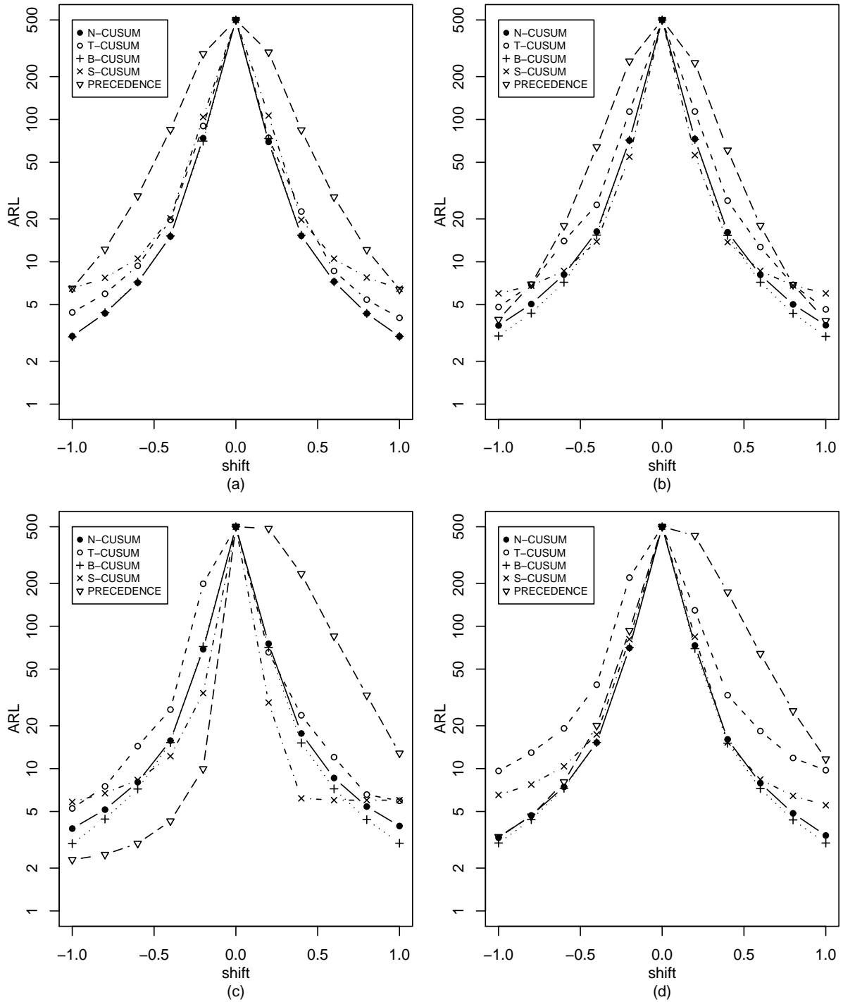
Figure 4: OC ARL values of five control charts when ARL_0 = 500 , M = 200 , m = 5 , and the actual IC process distribution is the standardized version of N(0,1) (plot (a)), t(4) (plot (b)), \chi^2(1) (plot (c)), and \chi^2(4) (plot (d)). Procedure parameters of the control charts are chosen to be the ones that minimize their OC ARL values when detecting each individual shift. Scale on the y -axis is in natural logarithm.
