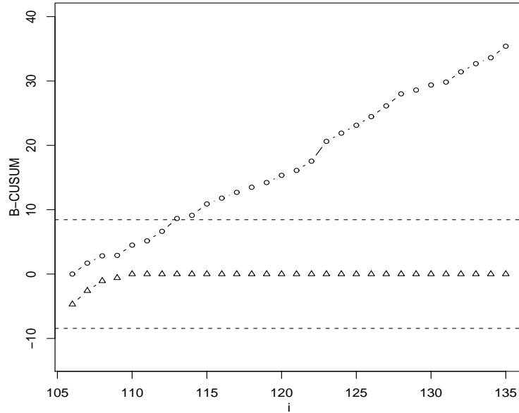
Figure 7: The B-CUSUM chart is applied to the exchange rate data. In the plot, the horizontal dashed lines denote its control limits, and the little circles and little triangles denote its upward and downward charting statistics, respectively.
